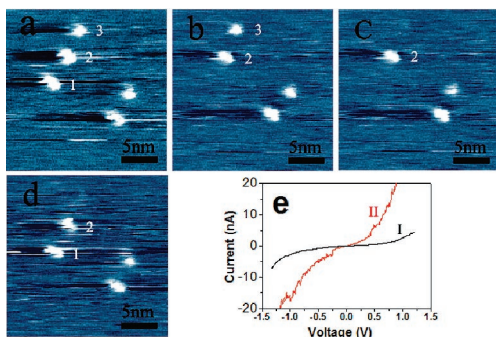
Figure 3. STM images of typical information dots pattern and the corresponding I-V curves. (a) Recording pattern composed of five information dots: pulsed voltage, +2.3 V; 3.0 ms. (b, c) Erasing the first and the second dots at position 1 and 3, respectively: pulsed voltage, -1.4 V; 3.0 ms. (d) Rewriting one information dot at position 1: pulsed voltage, +2.3 V; 3.0 ms. (e) Typical STM I-V curves in the unrecorded (curve I) and recorded region (curve II).
